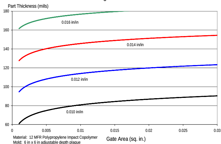
Contour Plots of Constant Mold Shrinkage as a Function of Gate Area and Part Thickness
